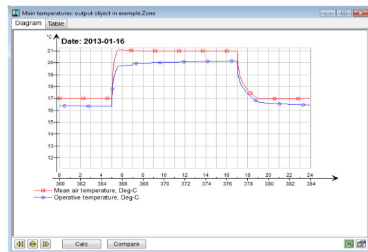
Figure 6 - Zone air temperature.
